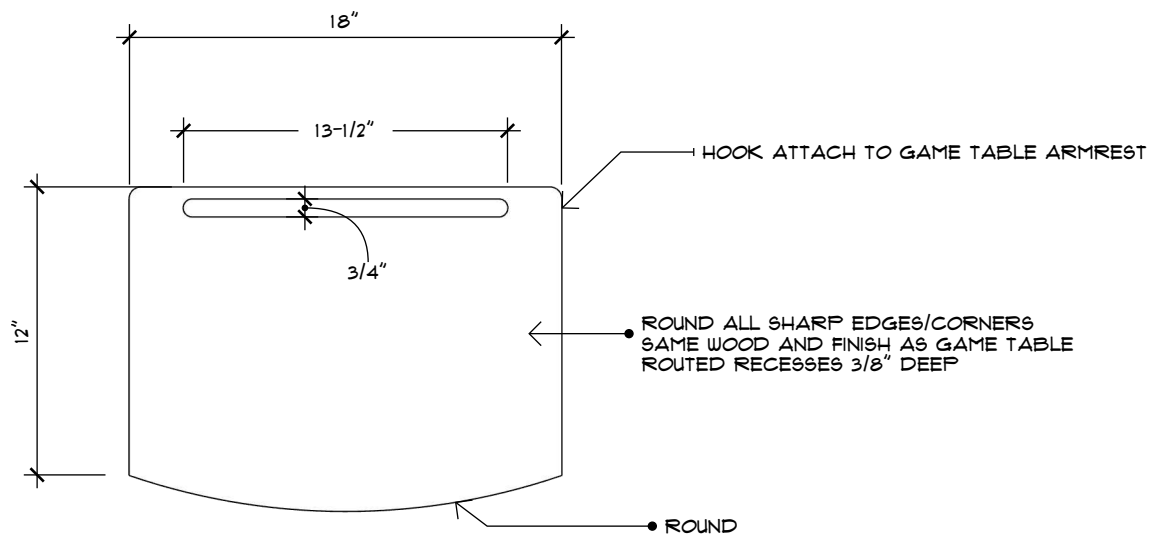
A PLAYER DESK DETAIL SCALE: 1-1/2" : 1'
