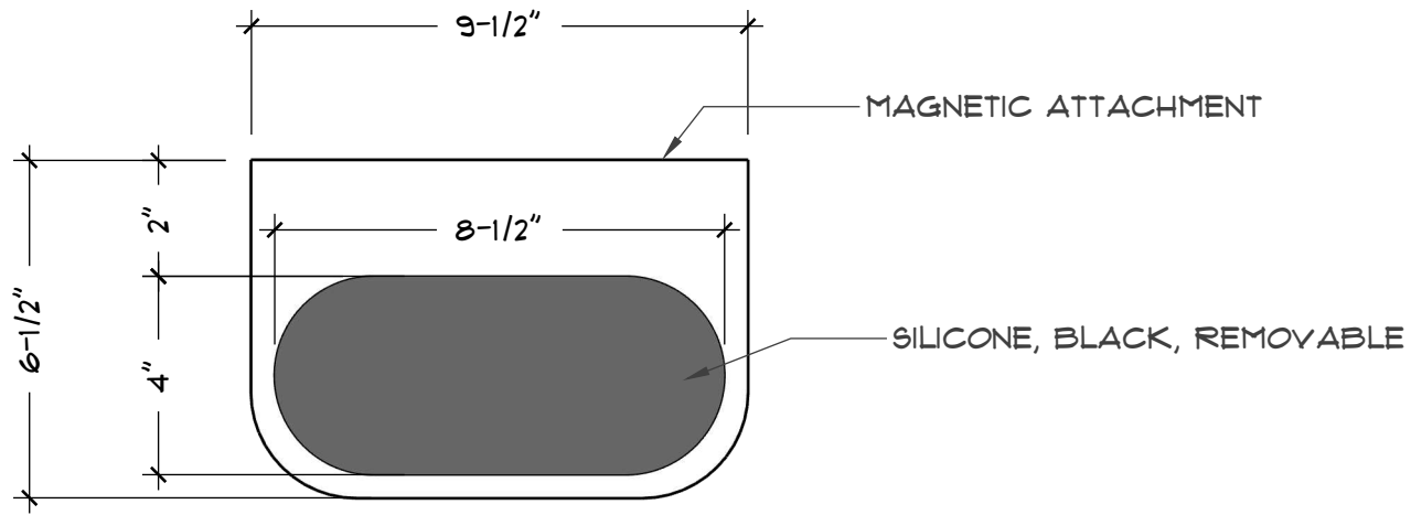
A DICE/PUZZLE TRAY DETAIL SCALE: 3" : 1"
