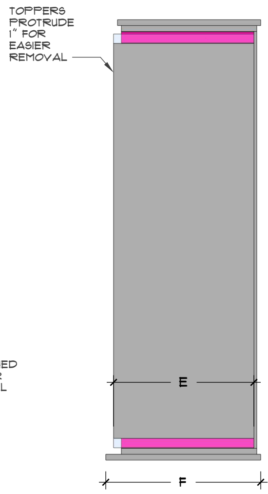
B TOPPER STAND, SIDE, SECTION VIEW SCALE: 1" : 1'
